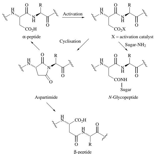
Scheme 1 Aspartimide formation during convergent N -glycopeptide synthesis. This side-reaction is depending on the chemical structure of the adjacent amino acid towards the C-terminal. For large oligosaccharides, aspartimide formation is predominant.
