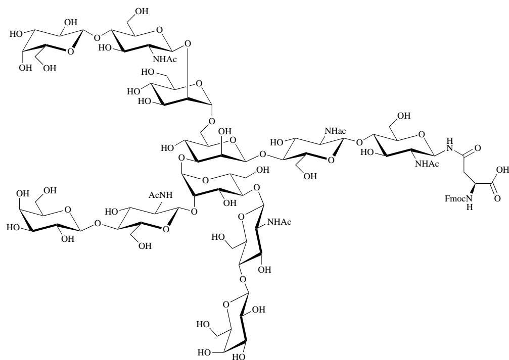
Scheme 4 Structures of di- and tri-antennary building blocks 38 and 39 ready for use in solid-phase peptide synthesis (SPPS)
