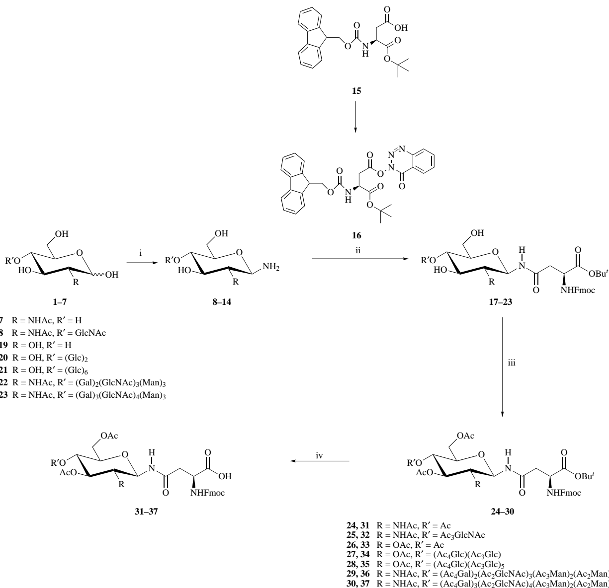
Scheme 3 Procedure for the synthesis of the oligosaccharide-asparagine building blocks 31–37 . Reagents and conditions : i, (NH 4 )HCO 3 ; ii, 16 (2 mol equiv.), DIPEA (1.2 mol equiv.), DMSO; iii, Ac 2 O-pyridine; iv, TFA (1 h).
